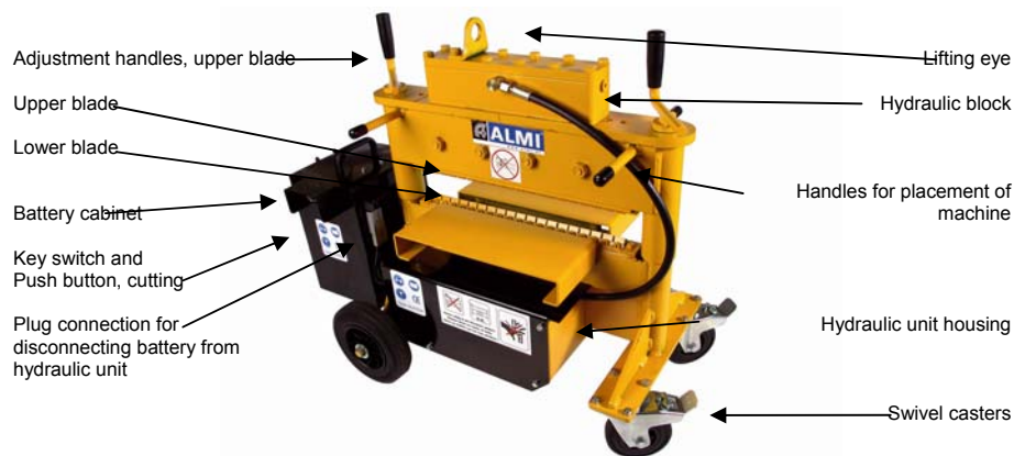
Figure 4.2-1: Construction of the machine
