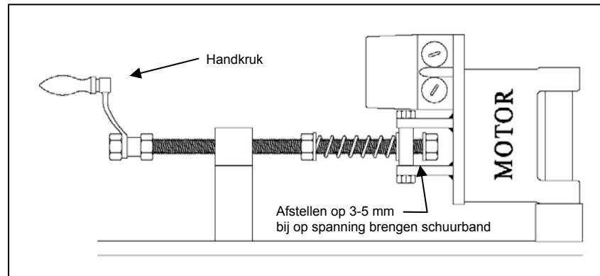
Figuur 4.6-3: Bandspanmechanisme
